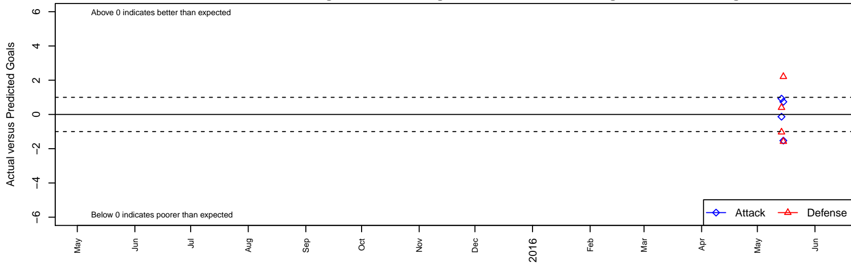
Bozeman Blitz Blue B99 Dots are actual minus expected GF (blue circles) and GA (red triangles). Blue line is smoothed change in attack strength. Red is smoothed change in defense strength.
